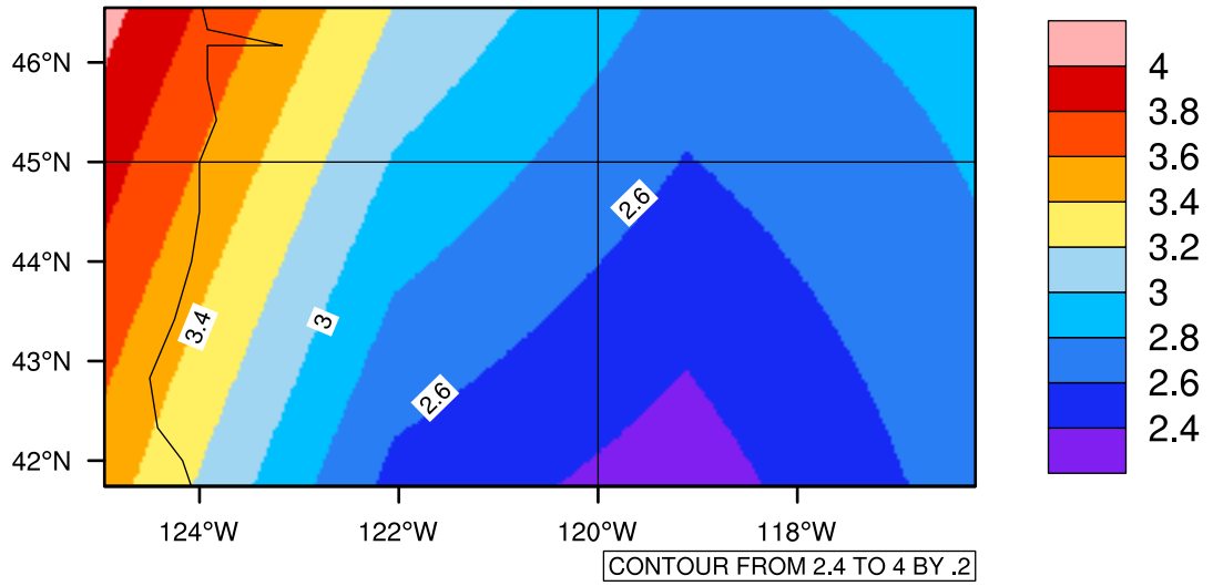
Yearly pr (mm/day) In 2030-2039 GFDL-ESM2M RCP85 - Oregon
