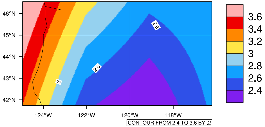
Yearly pr (mm/day) In 2040-2049 GFDL-ESM2M RCP85 - Oregon
