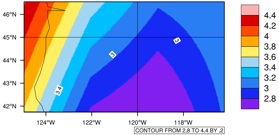
Yearly pr (mm/day) In 2050-2059 GFDL-ESM2M RCP85 - Oregon
