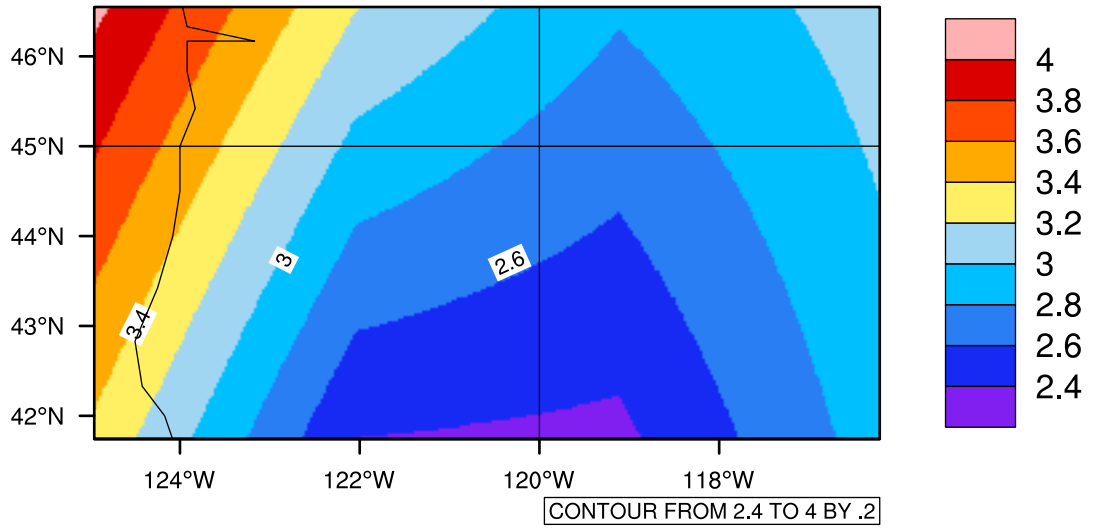
Yearly pr (mm/day) In 2080-2089 GFDL-ESM2M RCP85 - Oregon
