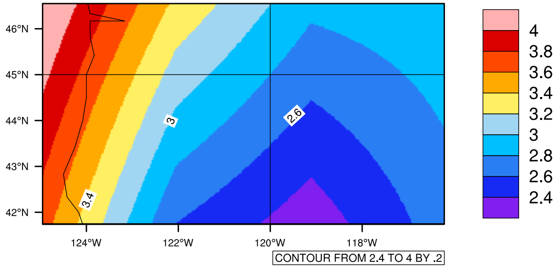
Yearly pr (mm/day) In 1975-2005 GFDL-ESM2M historical - Oregon
