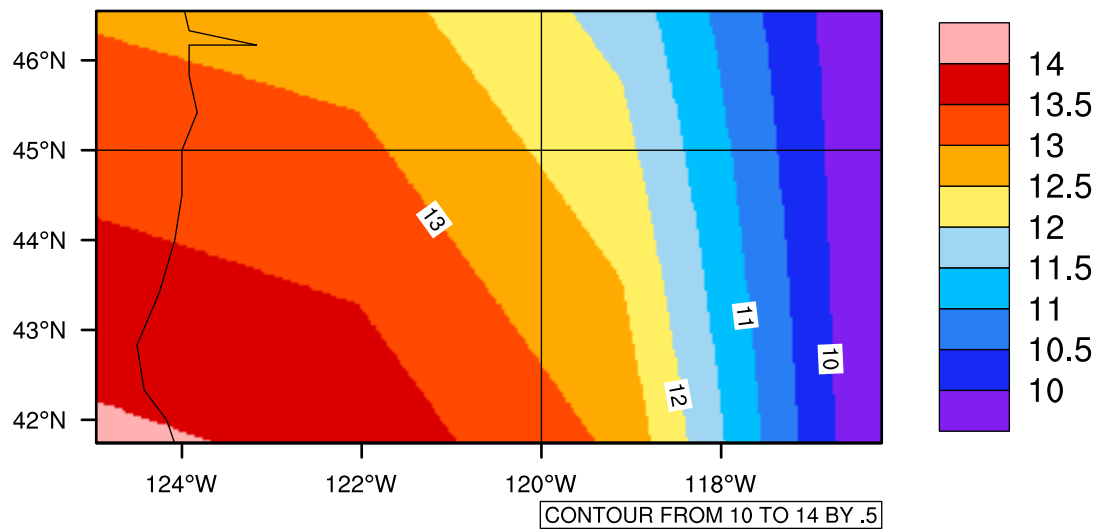
Yearly tasmax(c) In 2030-2039 GFDL-ESM2M RCP45 - Oregon
