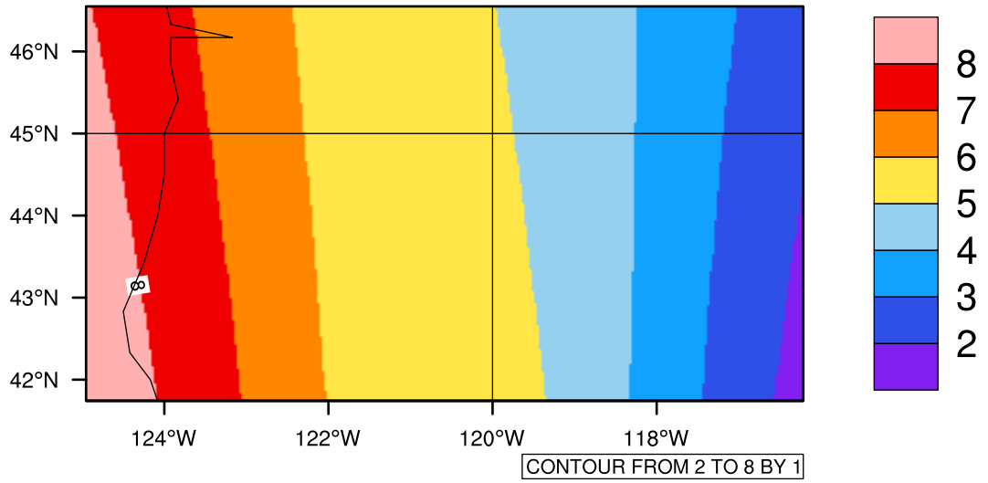
Yearly tasmin(c) In 2030-2039 GFDL-ESM2M RCP45 - Oregon
