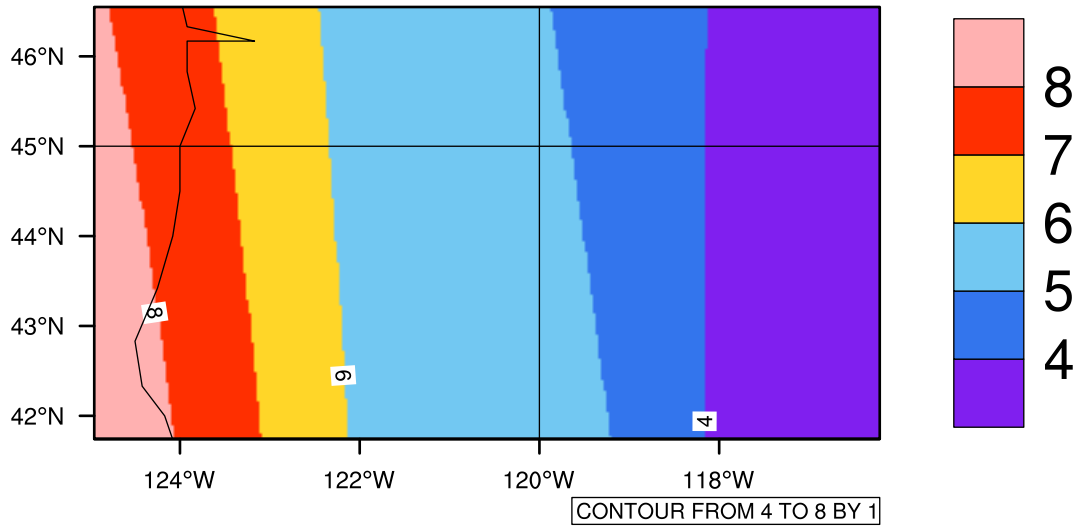
Yearly tasmin(c) In 2080-2089 GFDL-ESM2M RCP45 - Oregon
