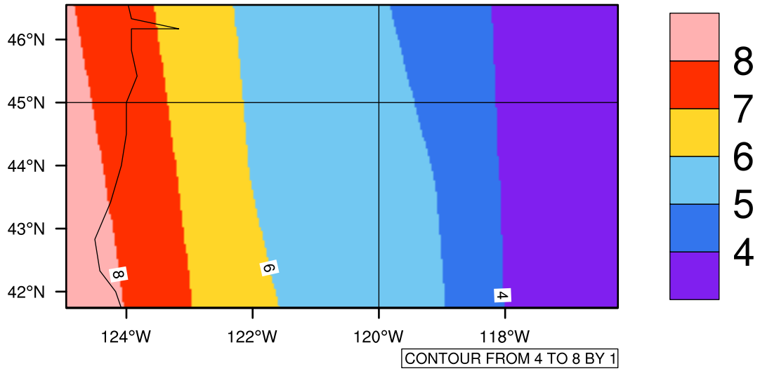
Yearly tasmin(c) In 2030-2039 GFDL-ESM2M RCP85 - Oregon
