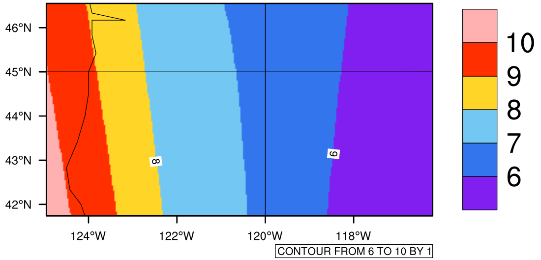
Yearly tasmin(c) In 2080-2089 GFDL-ESM2M RCP85 - Oregon
