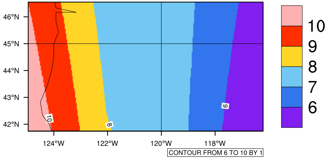
Yearly tasmin(c) In 2090-2099 GFDL-ESM2M RCP85 - Oregon
