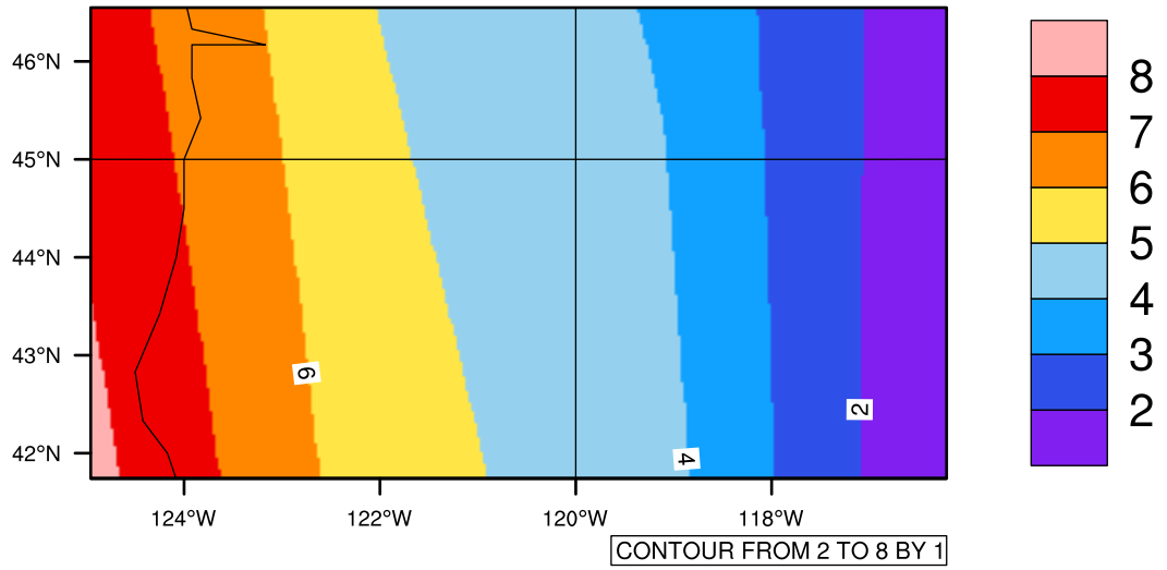
Yearly tasmin(c) In 1975-2005 GFDL-ESM2M historical - Oregon
