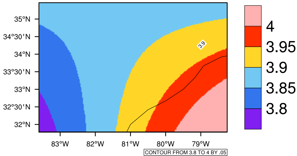
Yearly pr (mm/day) In 2020-2029 GFDL-ESM2M RCP45 - South Carolina
