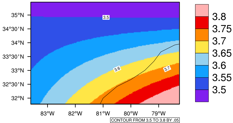
Yearly pr (mm/day) In 2030-2039 GFDL-ESM2M RCP45 - South Carolina
