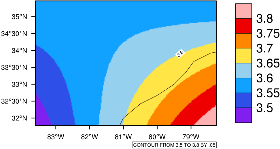
Yearly pr (mm/day) In 2040-2049 GFDL-ESM2M RCP45 - South Carolina
