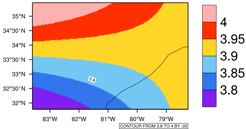
Yearly pr (mm/day) In 2050-2059 GFDL-ESM2M RCP45 - South Carolina
