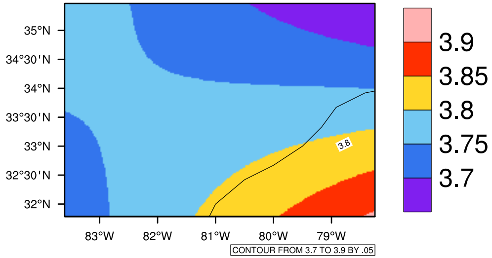
Yearly pr (mm/day) In 2060-2069 GFDL-ESM2M RCP45 - South Carolina
