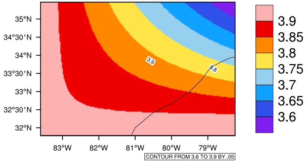
Yearly pr (mm/day) In 2080-2089 GFDL-ESM2M RCP45 - South Carolina
