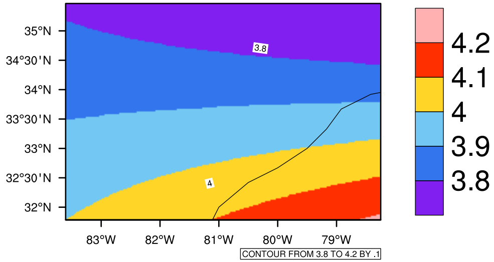
Yearly pr (mm/day) In 2020-2029 GFDL-ESM2M RCP85 - South Carolina
