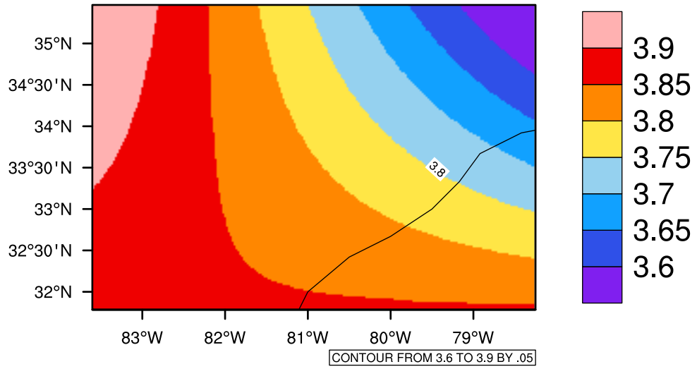
Yearly pr (mm/day) In 2040-2049 GFDL-ESM2M RCP85 - South Carolina
