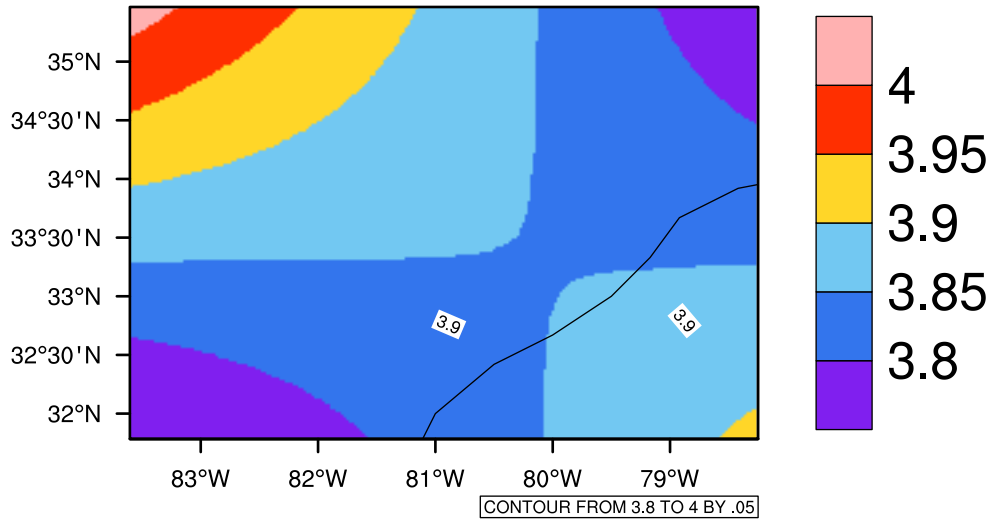
Yearly pr (mm/day) In 2050-2059 GFDL-ESM2M RCP85 - South Carolina
