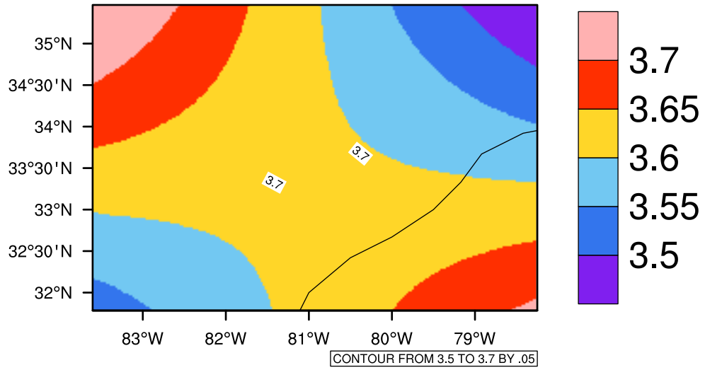
Yearly pr (mm/day) In 2070-2079 GFDL-ESM2M RCP85 - South Carolina
