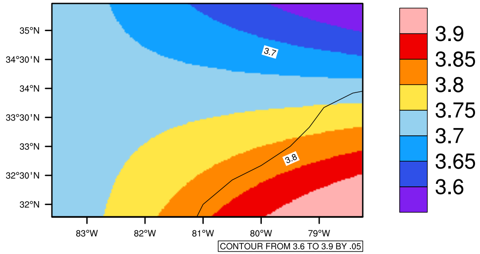
Yearly pr (mm/day) In 1975-2005 GFDL-ESM2M historical - South Carolina
