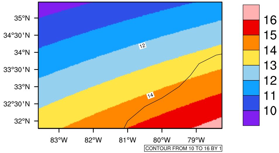
Yearly tasmin(c) In 2030-2039 GFDL-ESM2M RCP45 - South Carolina
