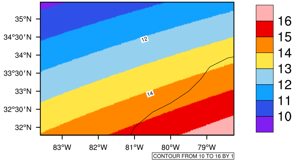
Yearly tasmin(c) In 2040-2049 GFDL-ESM2M RCP45 - South Carolina
