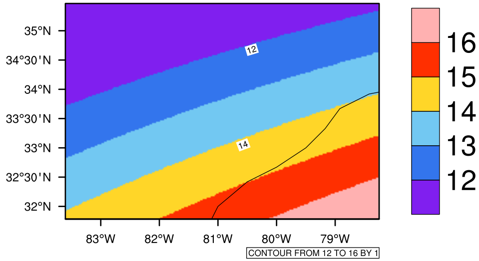
Yearly tasmin(c) In 2050-2059 GFDL-ESM2M RCP45 - South Carolina
