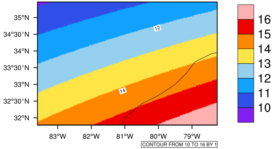
Yearly tasmin(c) In 2070-2079 GFDL-ESM2M RCP45 - South Carolina
