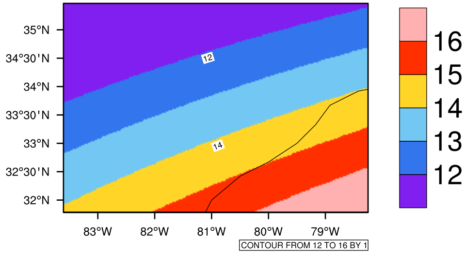
Yearly tasmin(c) In 2080-2089 GFDL-ESM2M RCP45 - South Carolina
