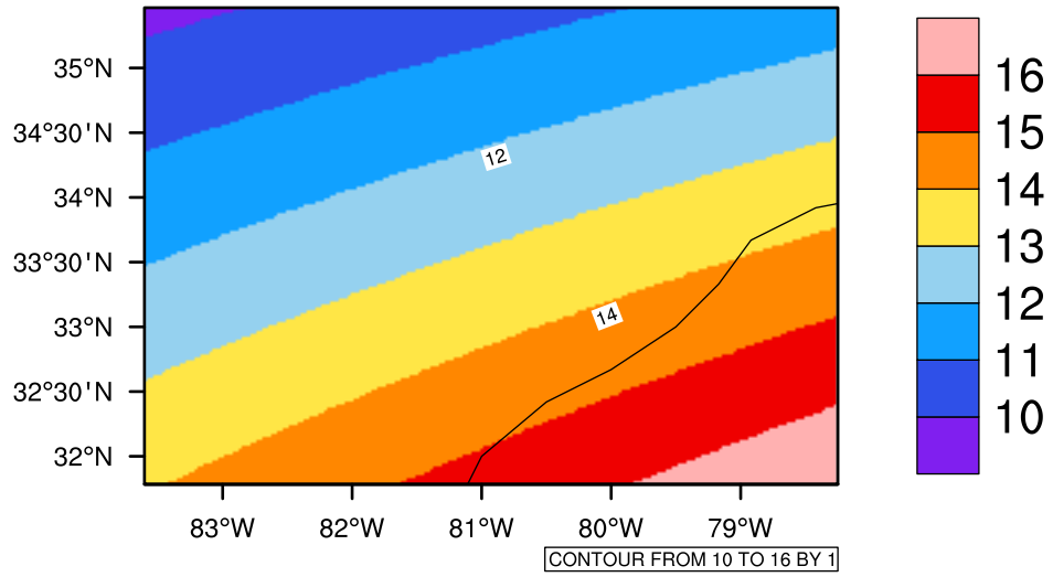
Yearly tasmin(c) In 2090-2099 GFDL-ESM2M RCP45 - South Carolina
