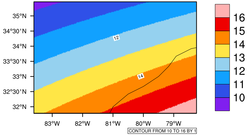
Yearly tasmin(c) In 2040-2049 GFDL-ESM2M RCP85 - South Carolina
