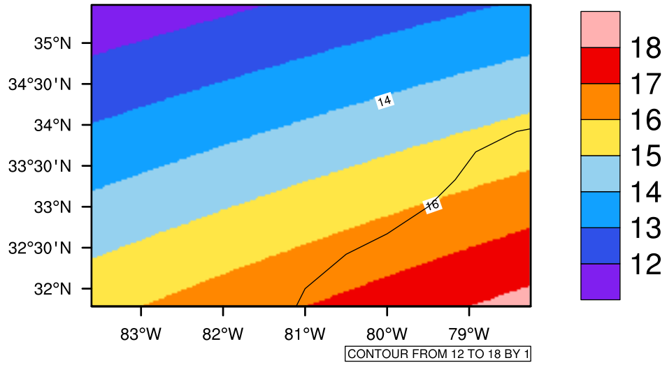
Yearly tasmin(c) In 2070-2079 GFDL-ESM2M RCP85 - South Carolina
