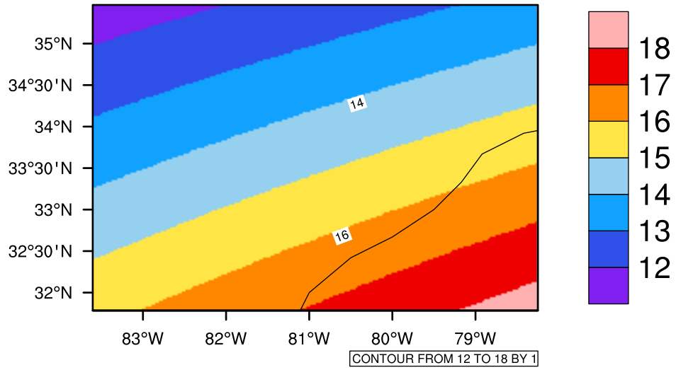
Yearly tasmin(c) In 2080-2089 GFDL-ESM2M RCP85 - South Carolina
