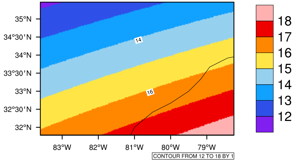
Yearly tasmin(c) In 2090-2099 GFDL-ESM2M RCP85 - South Carolina
