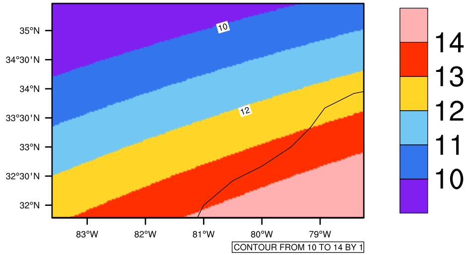
Yearly tasmin(c) In 1975-2005 GFDL-ESM2M historical - South Carolina
