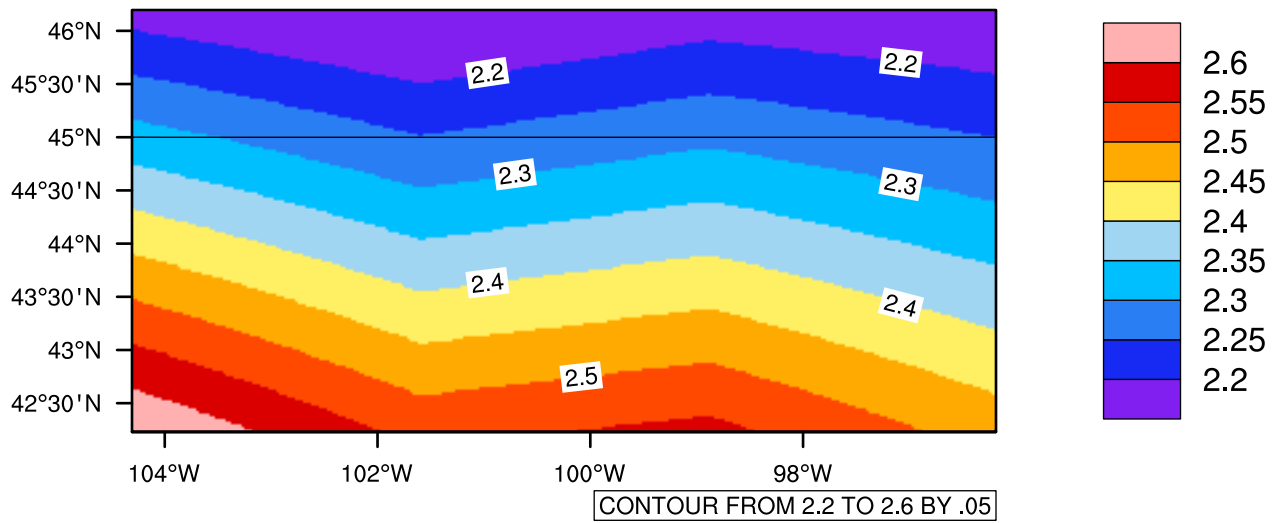
Yearly pr (mm/day) In 2020-2029 GFDL-ESM2M RCP45 - South Dakota
