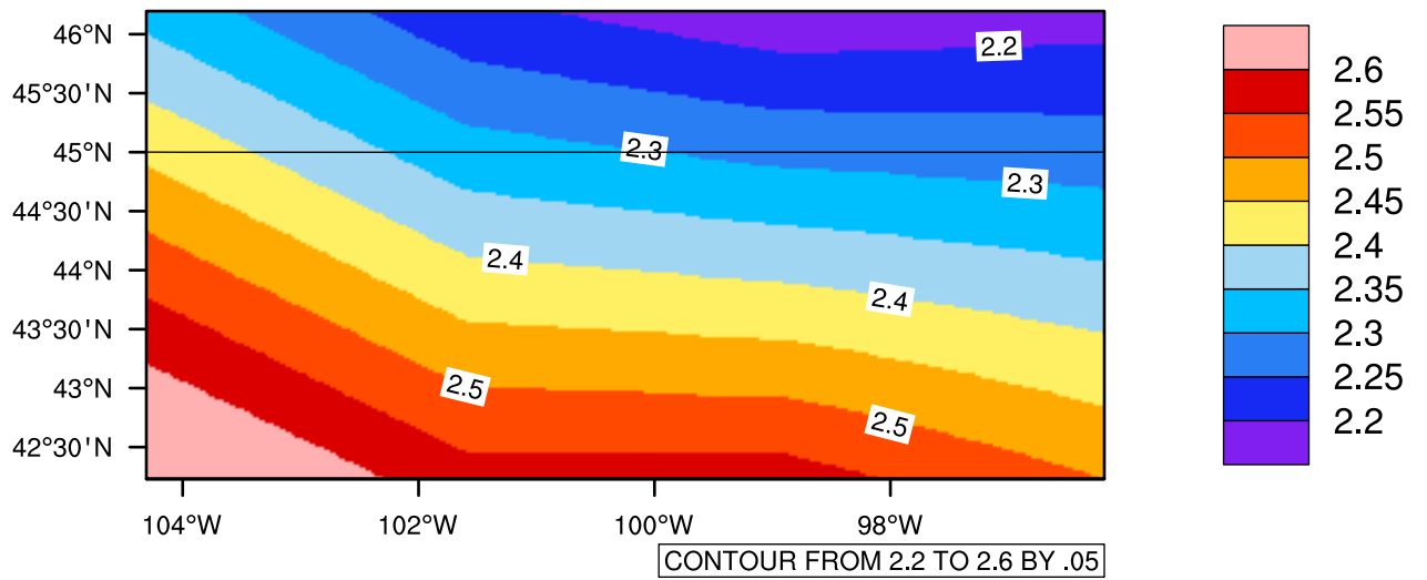
Yearly pr (mm/day) In 2040-2049 GFDL-ESM2M RCP45 - South Dakota
