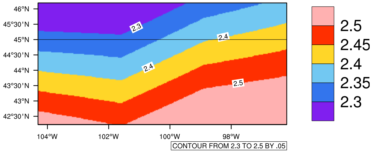
Yearly pr (mm/day) In 2050-2059 GFDL-ESM2M RCP45 - South Dakota
