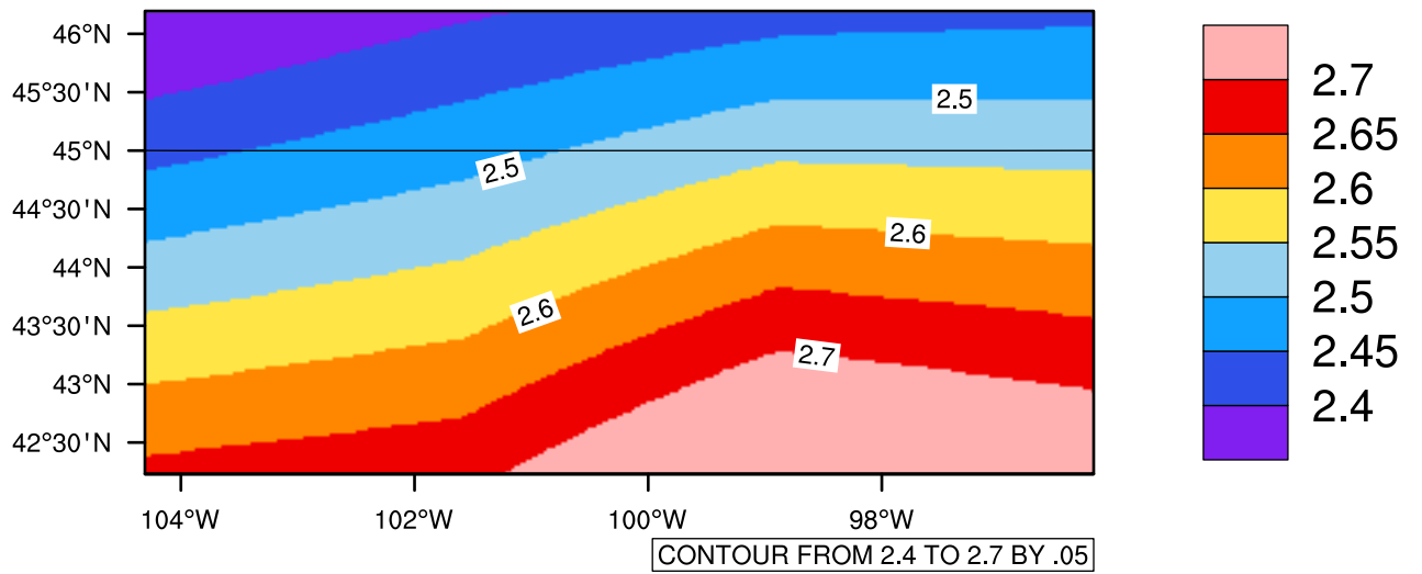
Yearly pr (mm/day) In 2060-2069 GFDL-ESM2M RCP45 - South Dakota
