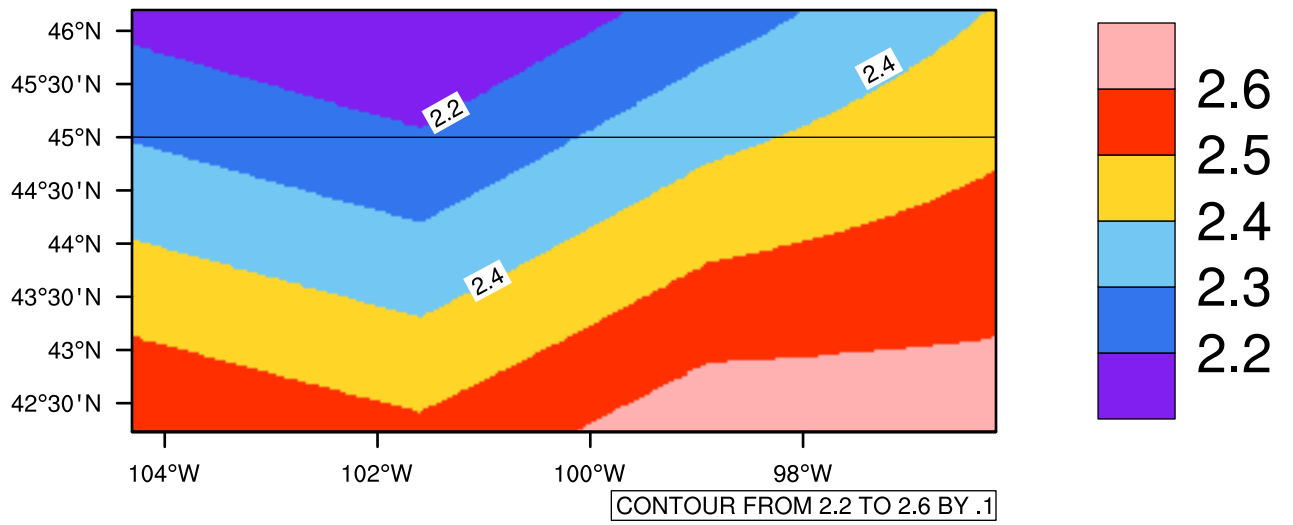
Yearly pr (mm/day) In 2070-2079 GFDL-ESM2M RCP45 - South Dakota
