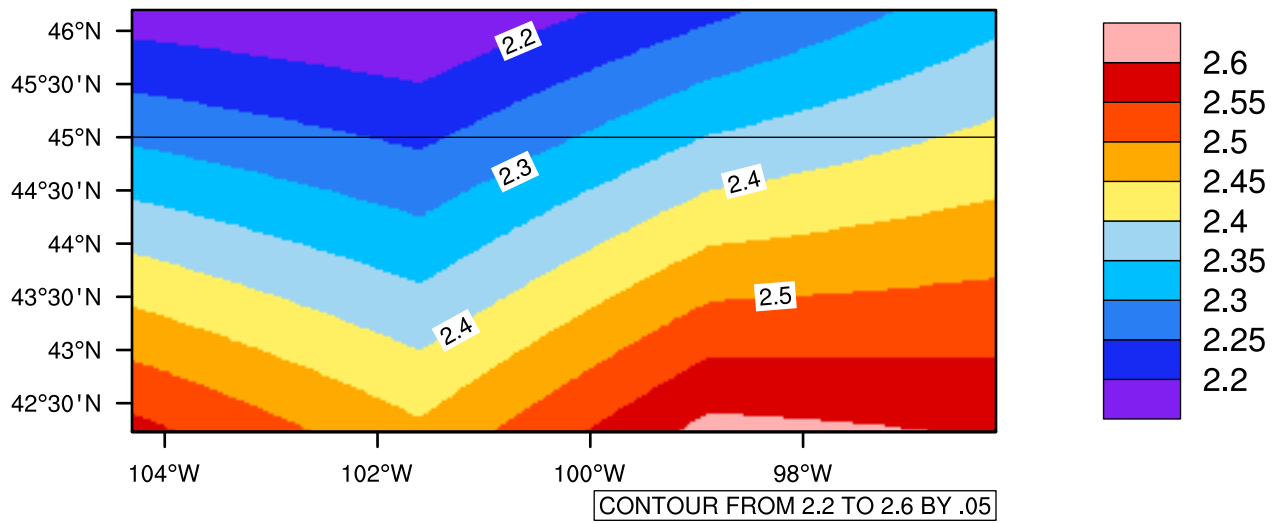
Yearly pr (mm/day) In 2080-2089 GFDL-ESM2M RCP45 - South Dakota
