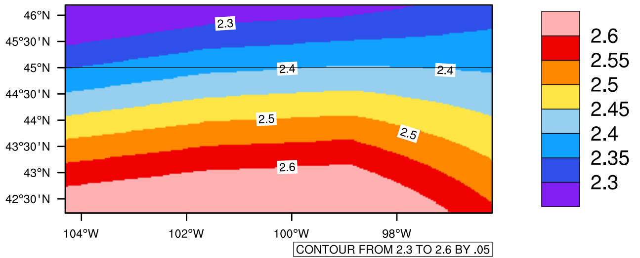
Yearly pr (mm/day) In 2020-2029 GFDL-ESM2M RCP85 - South Dakota
