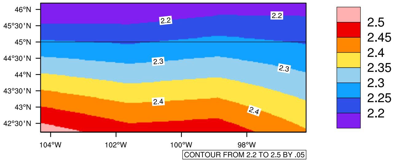
Yearly pr (mm/day) In 2050-2059 GFDL-ESM2M RCP85 - South Dakota
