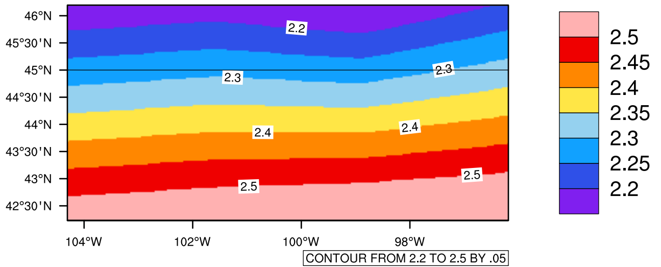
Yearly pr (mm/day) In 2060-2069 GFDL-ESM2M RCP85 - South Dakota
