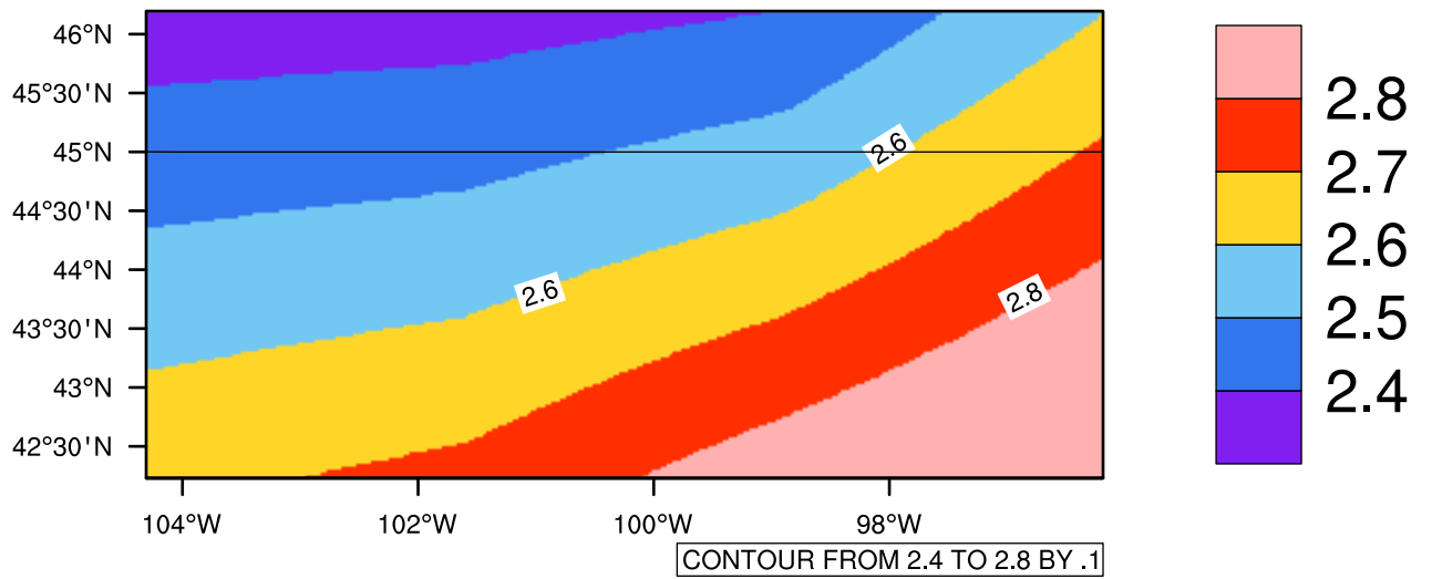
Yearly pr (mm/day) In 2080-2089 GFDL-ESM2M RCP85 - South Dakota
