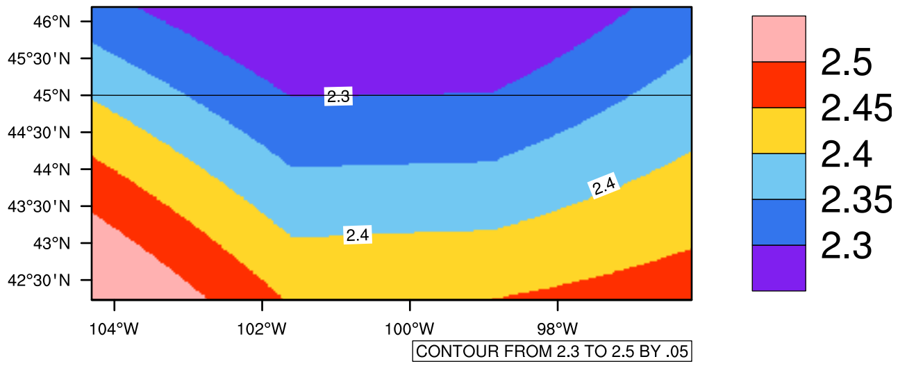
Yearly pr (mm/day) In 2090-2099 GFDL-ESM2M RCP85 - South Dakota
