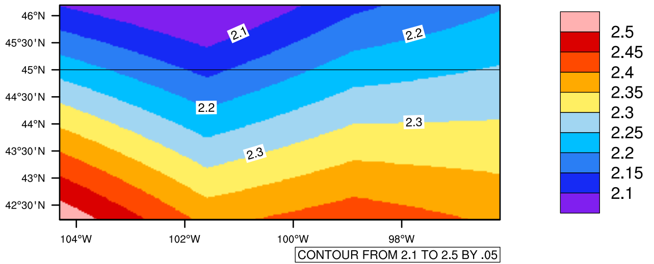
Yearly pr (mm/day) In 1975-2005 GFDL-ESM2M historical - South Dakota
