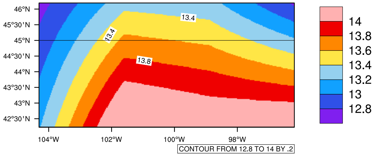
Yearly tasmax(c) In 2080-2089 GFDL-ESM2M RCP45 - South Dakota
