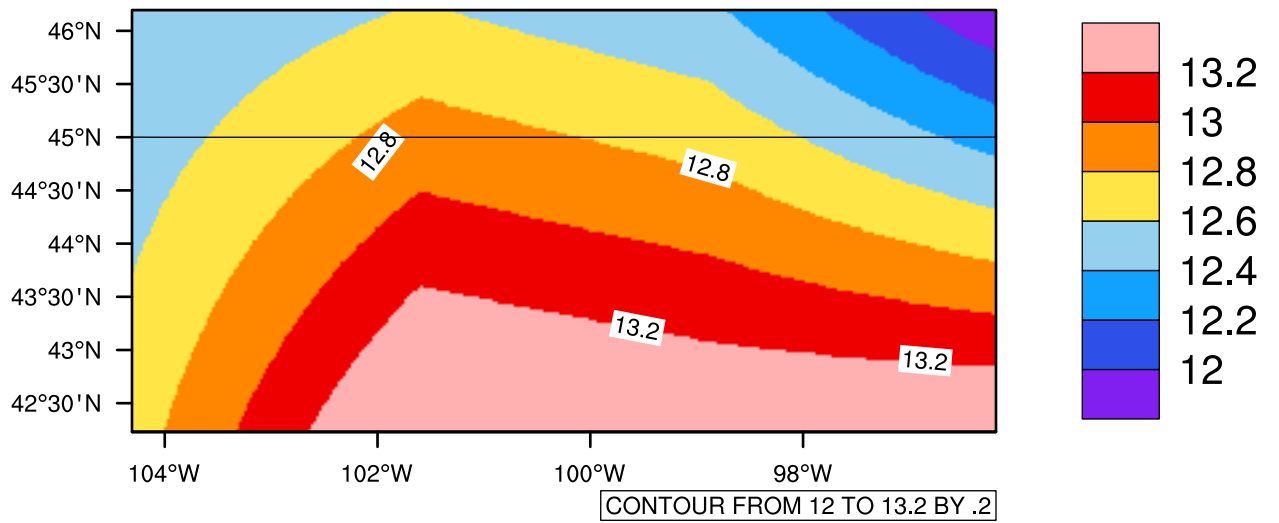
Yearly tasmax(c) In 2040-2049 GFDL-ESM2M RCP85 - South Dakota
