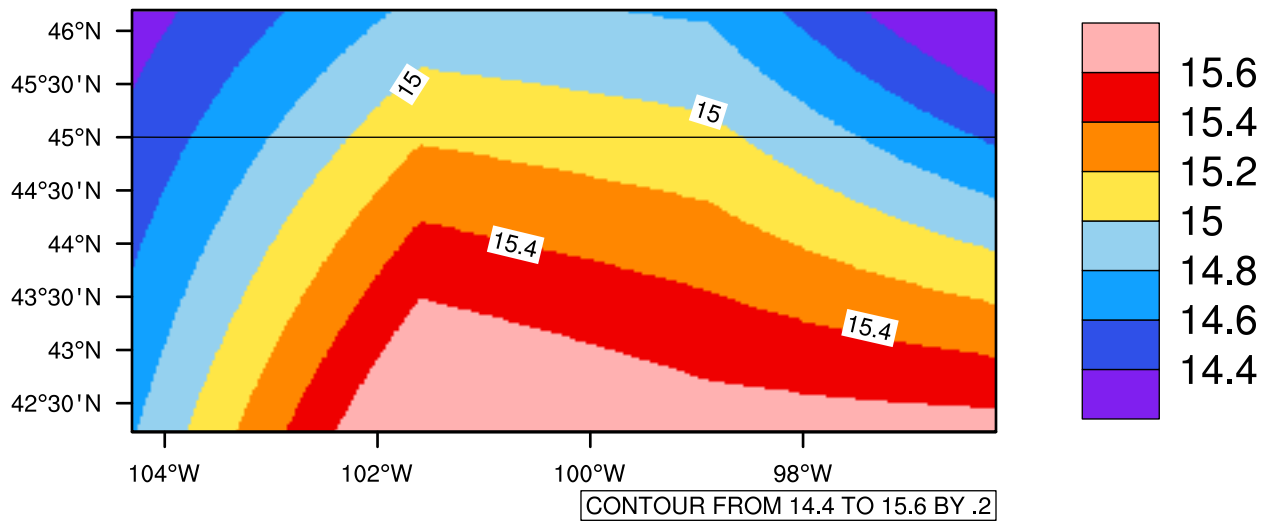
Yearly tasmax(c) In 2080-2089 GFDL-ESM2M RCP85 - South Dakota
