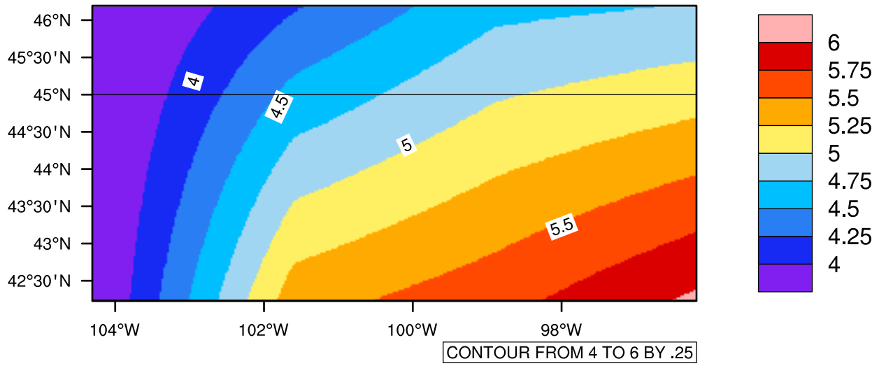
Yearly tasmin(c) In 2020-2029 GFDL-ESM2M RCP45 - South Dakota
